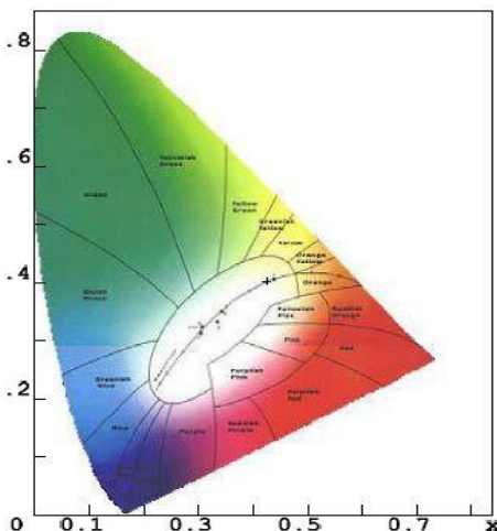
y CIE1931 Chromaticity Diagram
